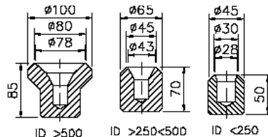
Gegenlager DF25/DF34/DF44 Opposite Support D25/DF34/DF44
