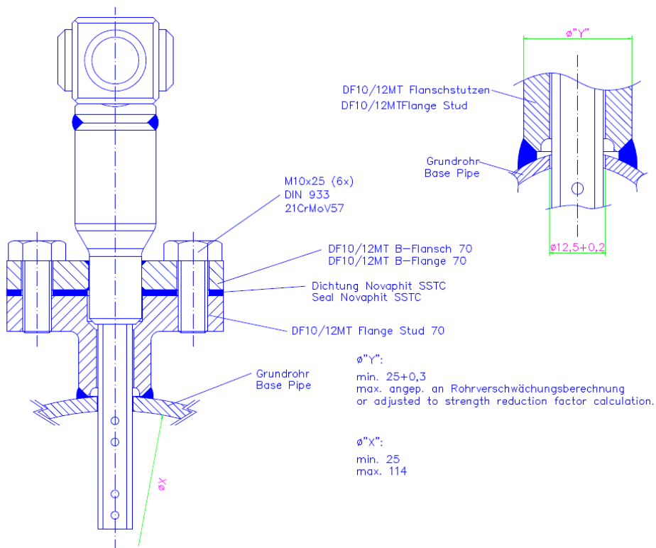
DF12 Flange-type
